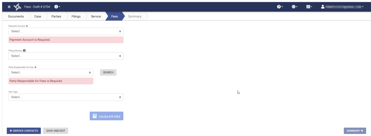
Figure 6.106 – Fees Page
