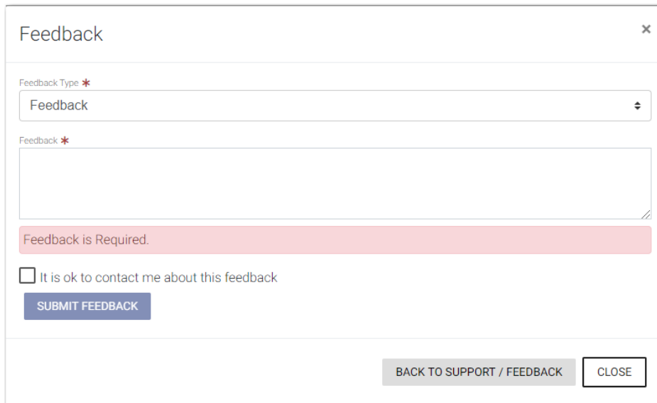
Figure 16.4 – Feedback Window
