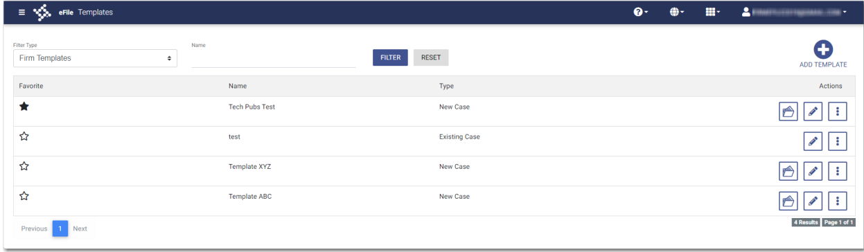
Figure 8.5 – Templates Page
