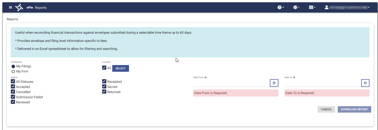
Figure 1.14 – Reports Page
