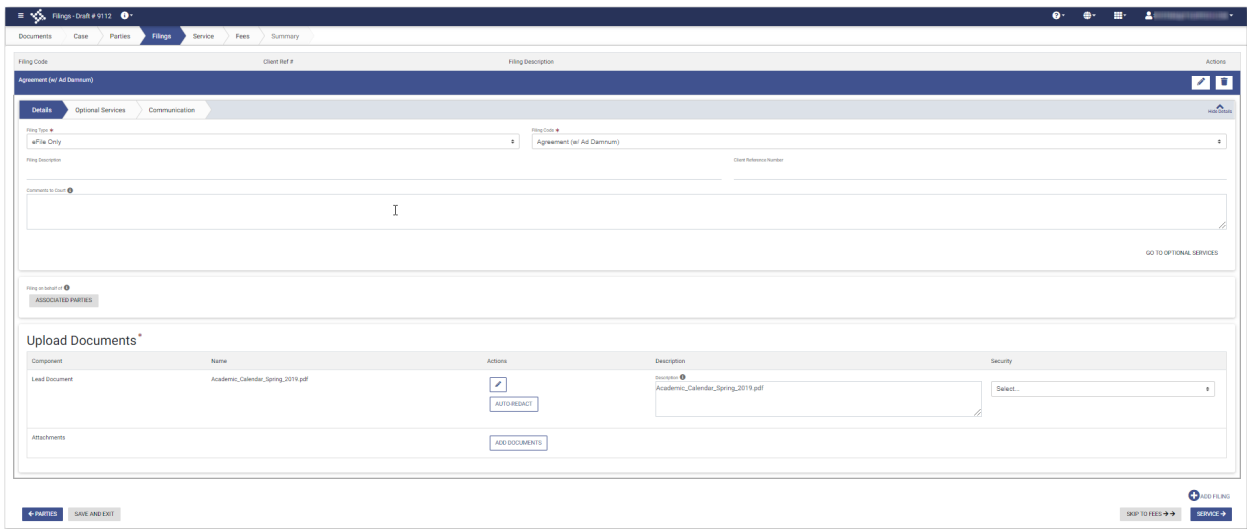
Figure 9.54 – Filings Page
