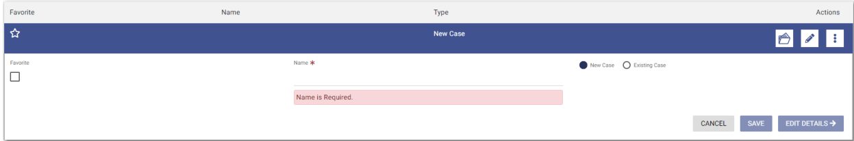
Figure 8.2 – Templates Pane
